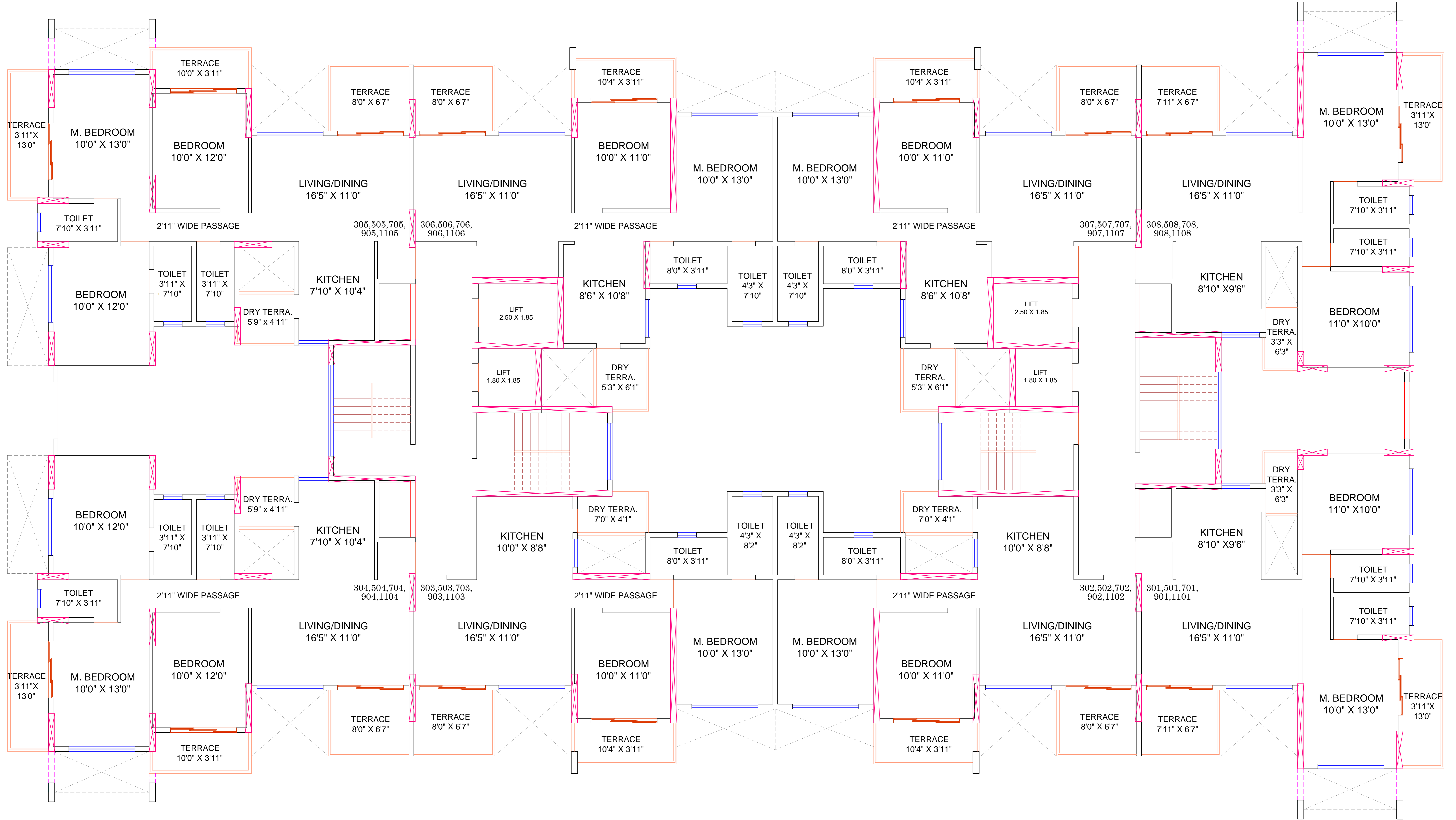
3RD, 5TH, 7TH, 9TH & 11TH FLOOR PLAN
