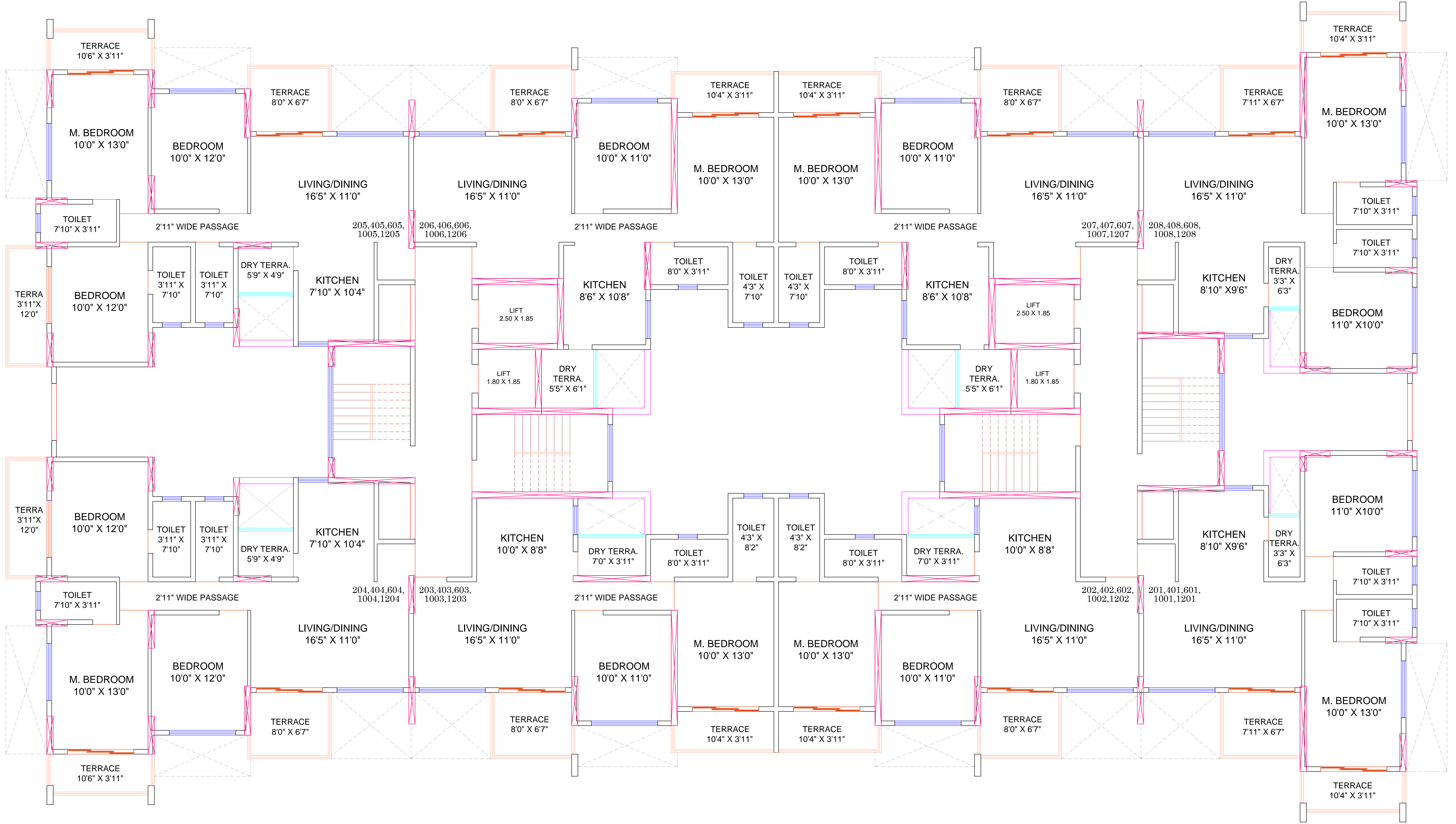
2ND, 4TH, 6TH, 10TH & 12TH FLOOR PLAN
